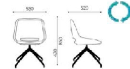
SS.039.SPG - pyramidal base cr./black
