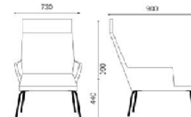
SS.042.24.L - lounge 4 eggs
