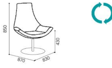
SS.042_3.A4S - Armchair Round base Polished steel swivel
