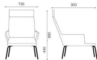
SS.042_2 - Armchair 4 legs Chromed
