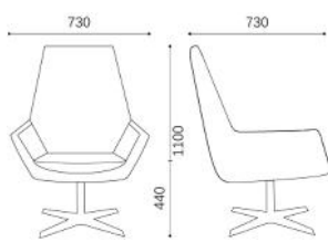
SS.042_1.4S - Armchair 4 star metal base Polished Chromed swivel
