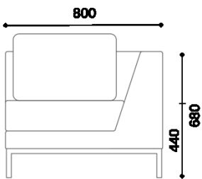
SS.007.1C - Corner element
