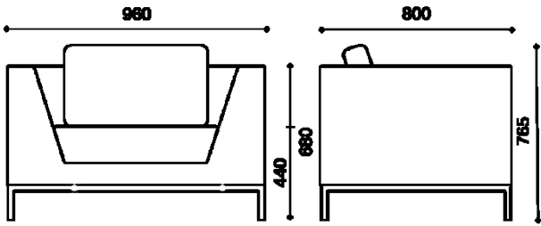
SS.007.1S - Armchair
