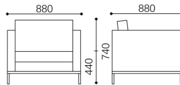
SS.022.1S - Sofa single seat
