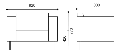
SS.016.1A - Armchair high back
