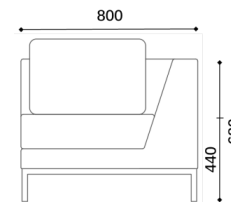
SS.007.1C - Corner element
