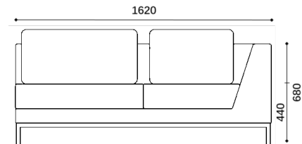
SS.007.2P.L-R - 2 seater element R/L hand
