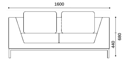
SS.007.2S - Sofa 2 seater
