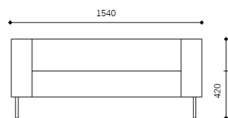
SS.016.2S - 2 seater sofa
