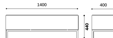
SS.007.PR - Rectangular bench
