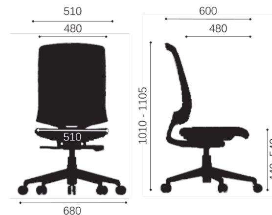
SS.MIR.SB – Armless chair
