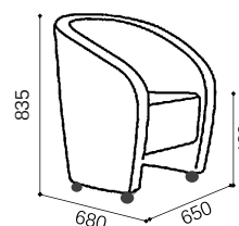
SS.038.1.R - Armchair with castors
