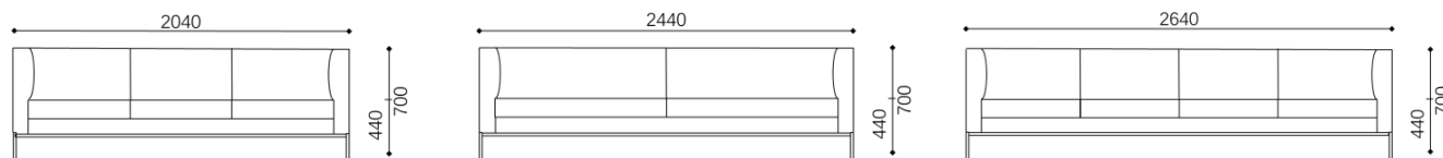
SS.012.3S3 - Sofa 3 seater large, 3 cushions
