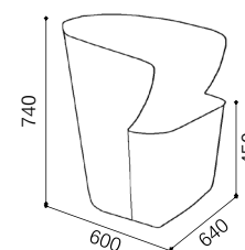
SS.038.3.P - Armchair with glides
