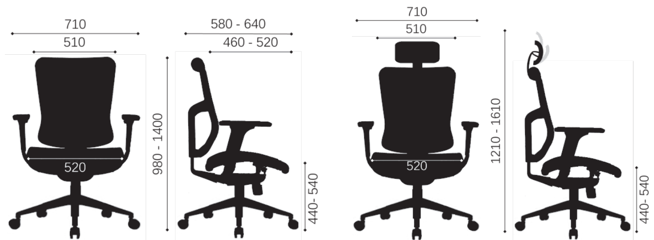
SS.PAK.A – Mid back armchair
