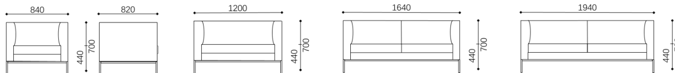
SS.012.1S - Armchair
